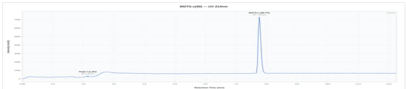
MOTS-C 40mg - PUP-MS40-001: UV Chromatogram
