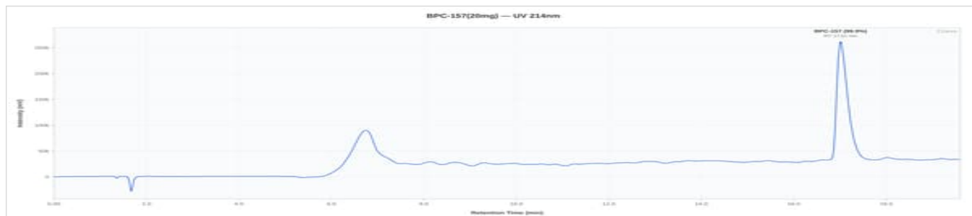
BPC-157 20mg - PUP-BC20-001: UV Chromatogram
